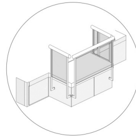
Node of a terrace protection
